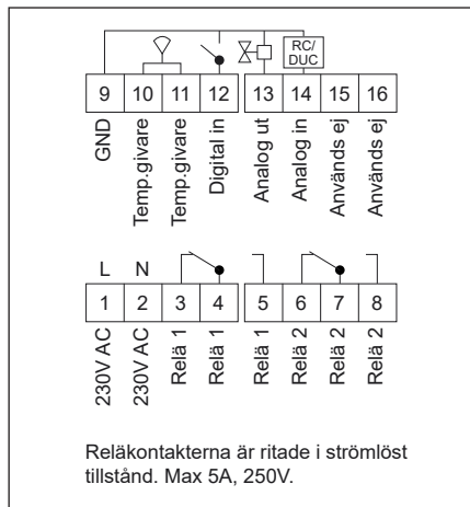
FIG. 3 (CFA-230V)
