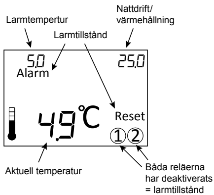
FIG. 2 (CFA-24V)
