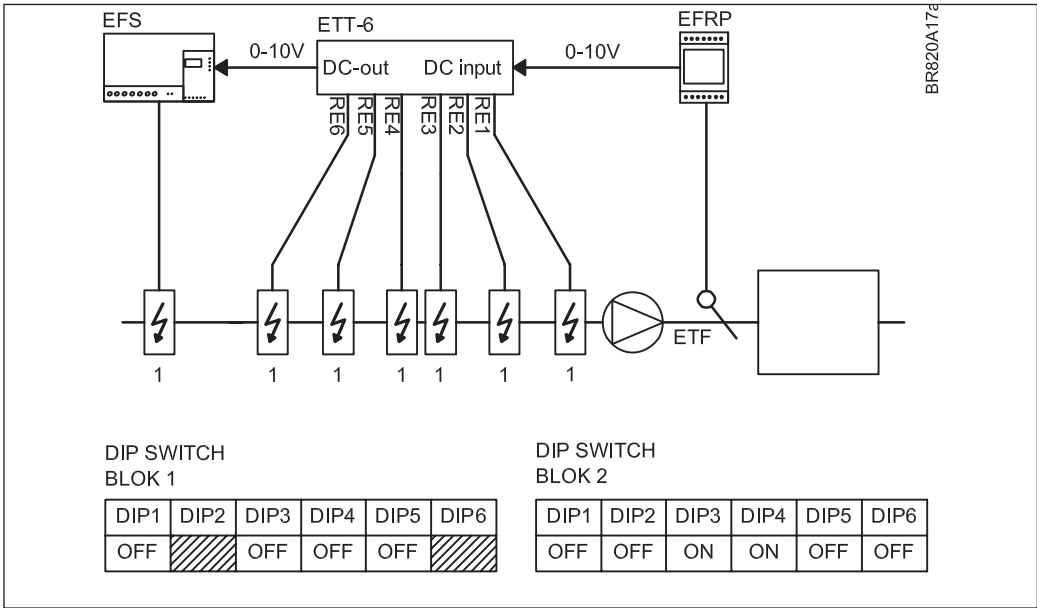
Fig. 6 - Uniform power output
