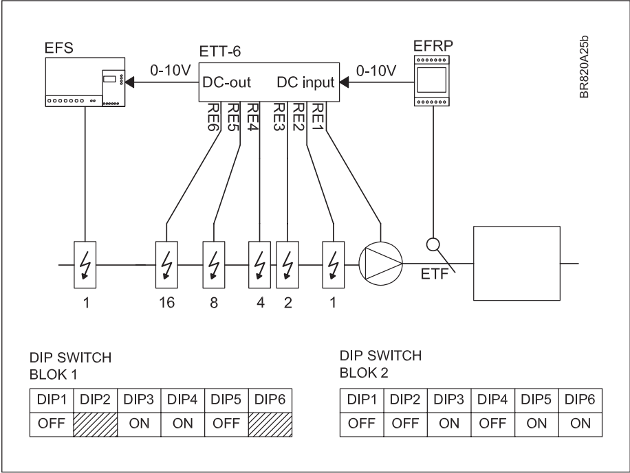
Fig. 14 - Fan operation, binary power output
